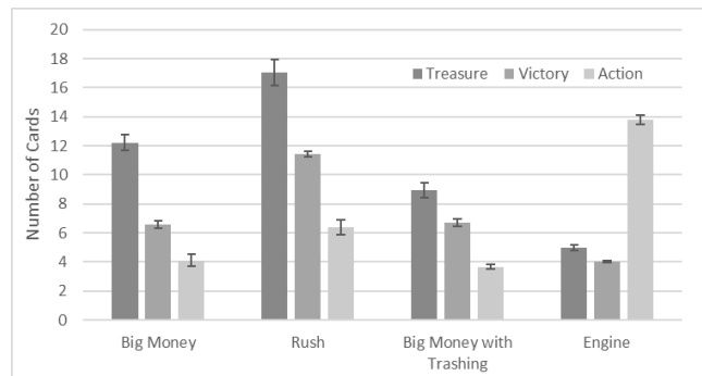
Figure 2: Average deck composition by card type of each of the four agents developed.
